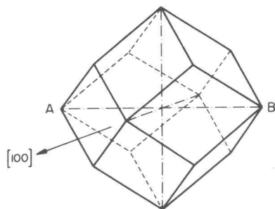
Fig. 2. Schematic representation of the rhombic dodecahedron single-crystal sample of almandine-garnet used in this study.
